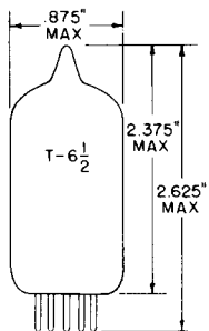
GLASS BULB
