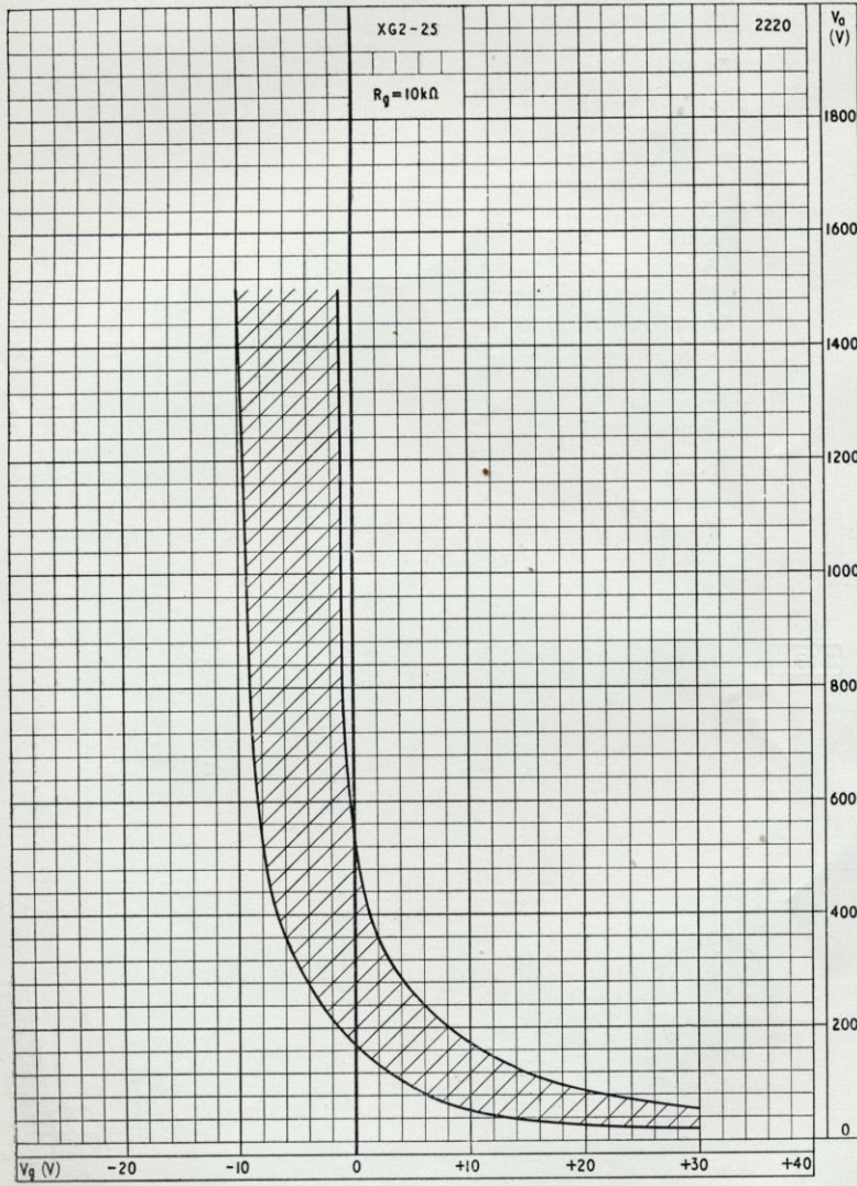
CONTROL CHARACTERISTIC
