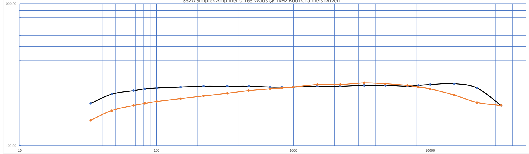
832A Simplex Amplifier 0.165 Watts @ 1kHz Both Channels Driven
