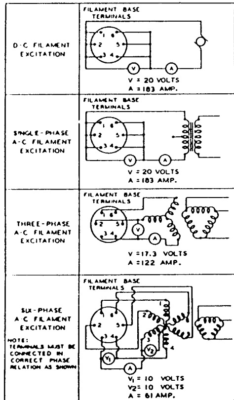
FILAMENT CONNECTIONS AND EXCITATION CIRCUITS
